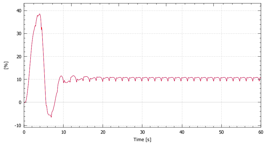
Torque coef. (CQ)
